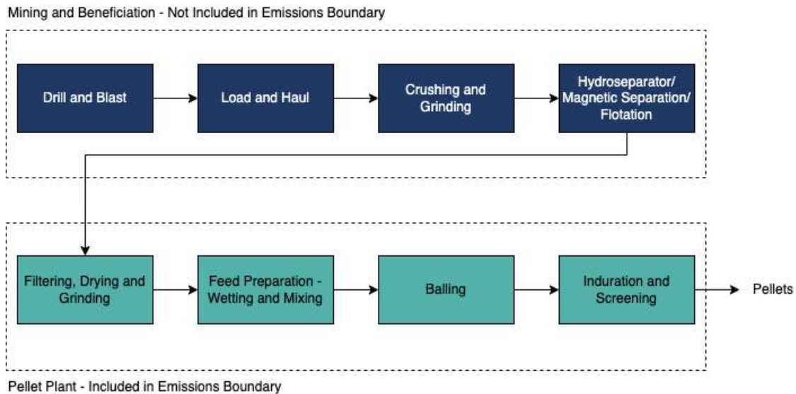
Exhibit 15. Pellet Plant Boundary
