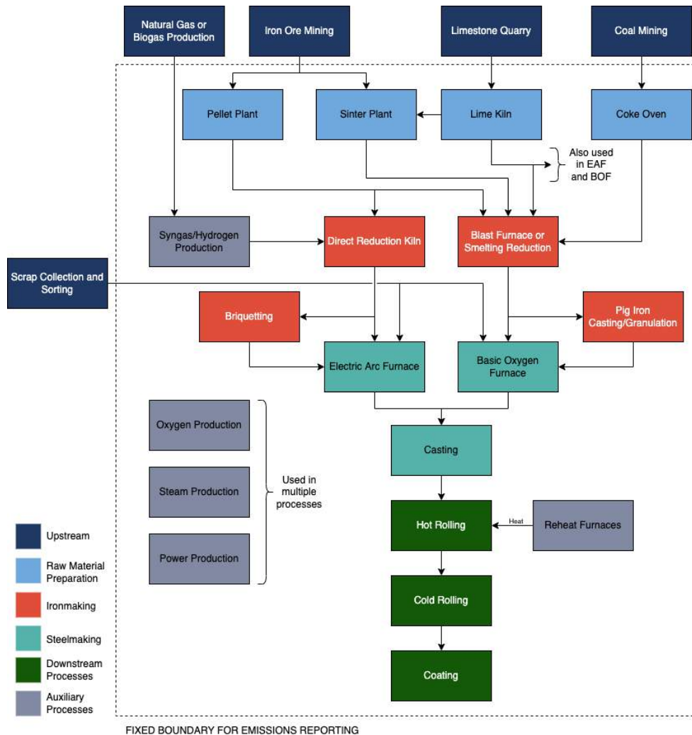
Exhibit 14. Fixed System Boundary of the Sustainable STEEL Principles
